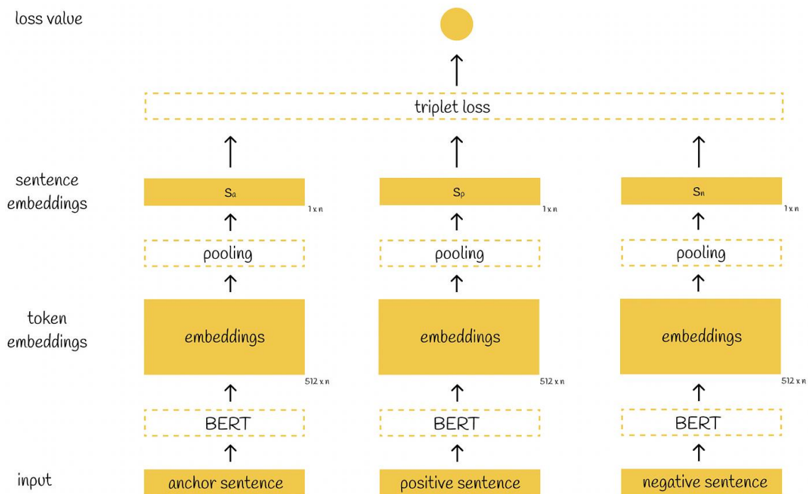
Figure 5.1.1: Sentence-BERT Diagram
